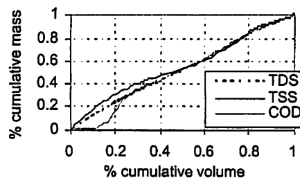
Fig. 5. Cumulative mass plot showing no first flush effect.
