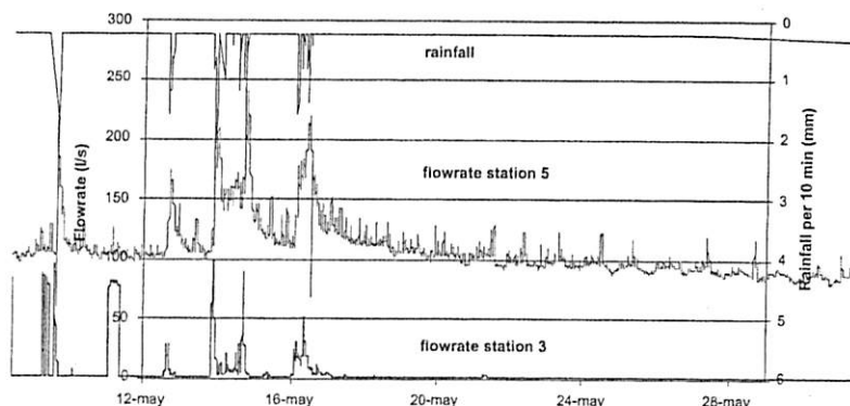
Fig. 3. Rainfall-runoff measures for stations 3 and 5
